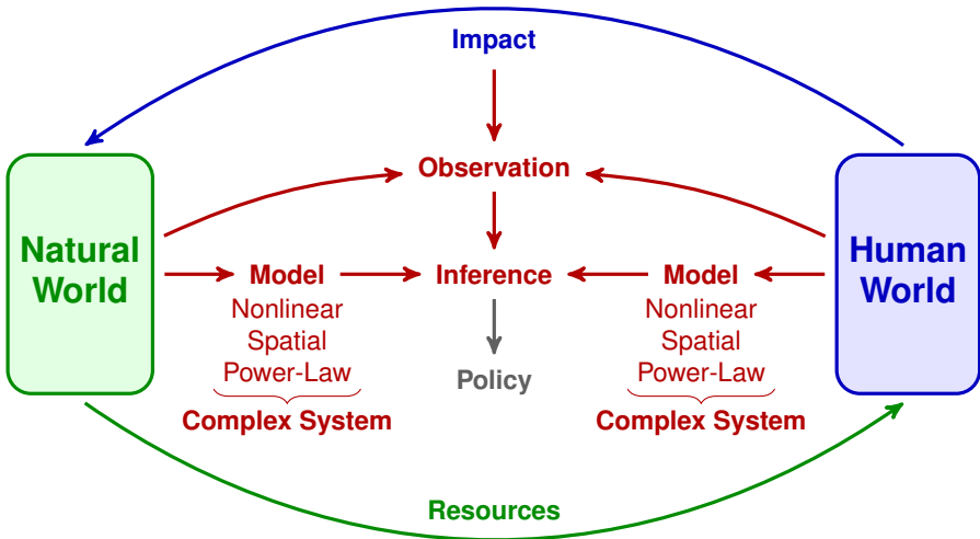
Fig. 1.1. AN OVERVIEW: Human / societal / economic systems (right) draw resources from and have an impact on natural / ecological / environmental systems (left). Both domains contain many examples of systems which exhibit one or more elements of non-linearity and spatial interaction, leading to complex-systems and power-law behaviours. Observations of one or more systems are combined with models in an inference process, leading to deeper insights and (ideally) better policy. The red portions are the focus of this text, with the blue, green, and grey components illustrating the broader, motivating context.
