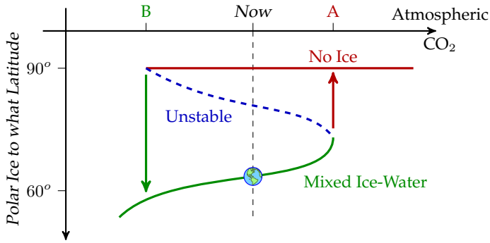
Fig. 2.1. STABLE CLIMATE STATES AS A FUNCTION OF ATMOSPHERIC CARBON-DIOXIDE: The earth may have no ice (top) or may have polar ice to some latitude (middle); the arrows indicate the discontinuous climactic jumps (“catastrophes”). Although obviously an oversimplification of global climate, the effects illustrated here are nevertheless real.
